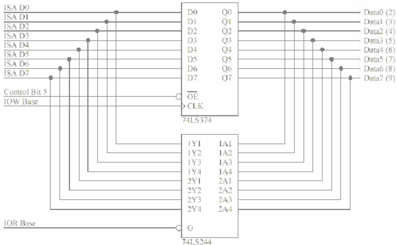
Standard Parallel Port Bi-Directional Operation
