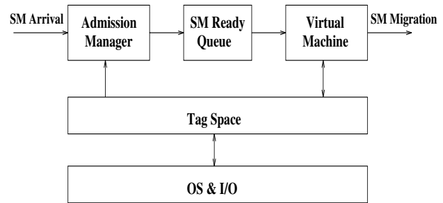
Figure 1. Node Architecture
